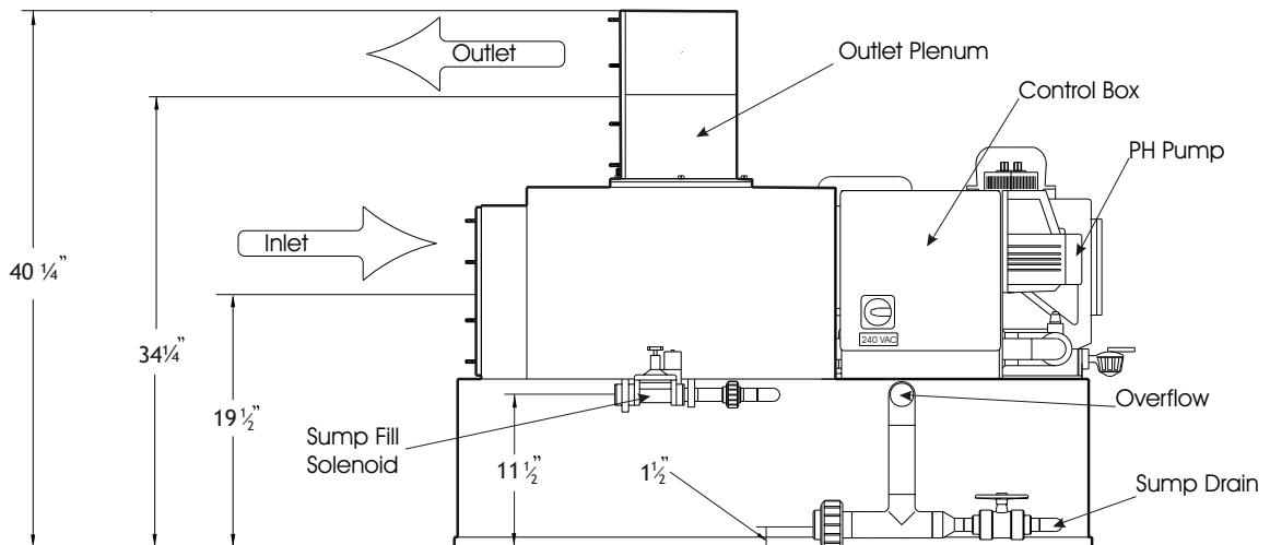
Side View
